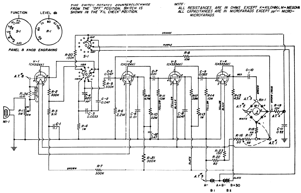
Wiring Diagram for Type 1555-A Sound-Survey Meter
